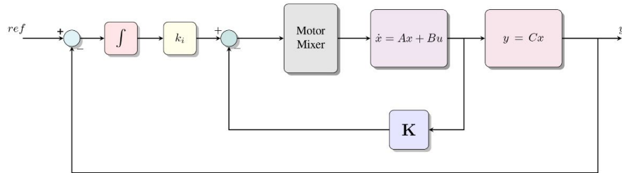
Figure N° 11. Complete representation of quadcopter state feedback. Source: Own elaboration, 2025.
